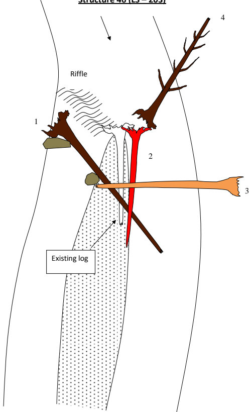
Structure 46 (LS - 203)
