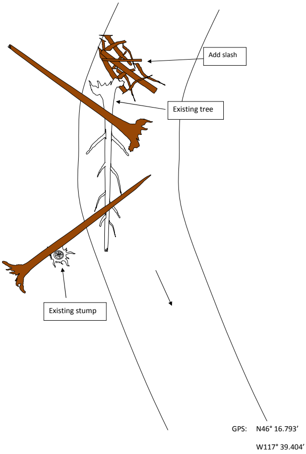
Structure 48 (TRI - 201)
