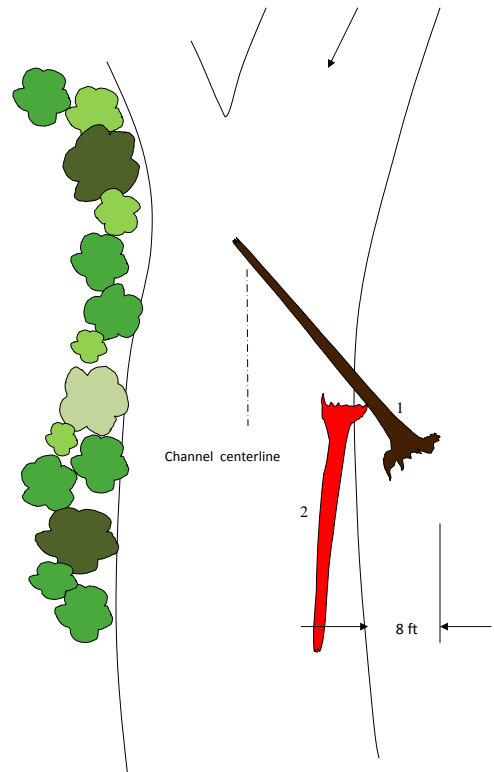
Structure 3 (CH-1)
