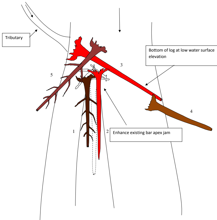
Structure 38 (BAJ-4)
