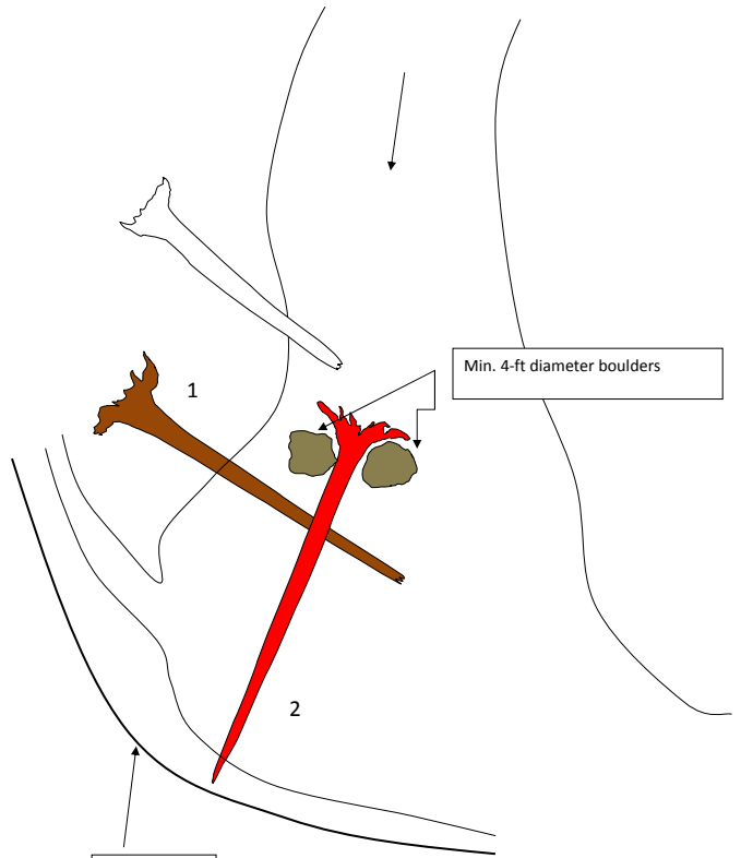
Structure 33 (T - 4)
