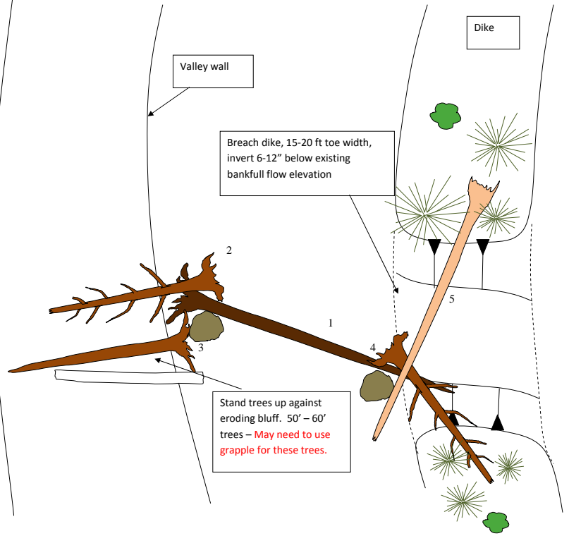
Structure 37 (SP-9)
